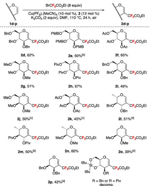
Scheme 4. Synthesis of Fluorinated Glycal Derivatives a
